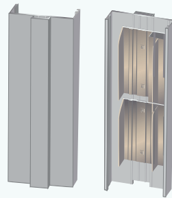
TYPE I FRAME SYSTEM
